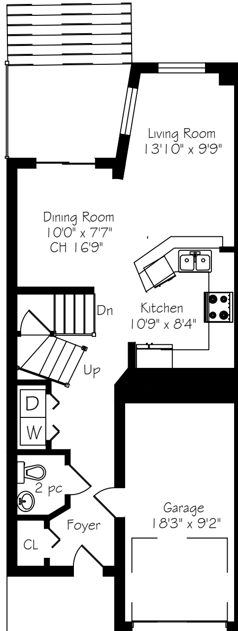
Main Floor 615 Square Feet + 188 Garage
